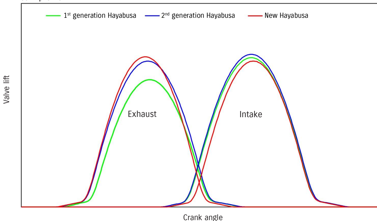
Cam profile
