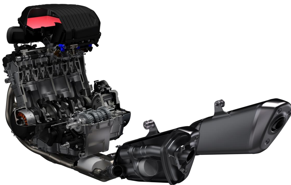
Engine cutaway
